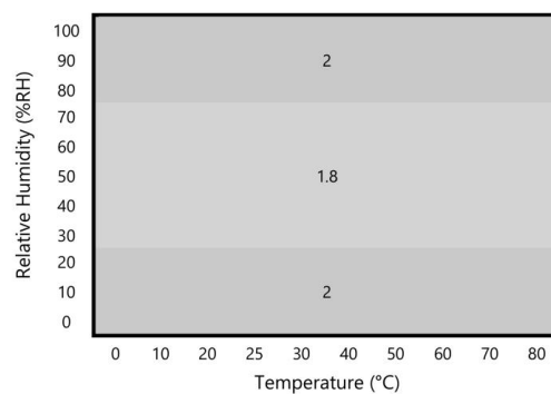
4. Typical RH accuracy corresponding to the temperature.
