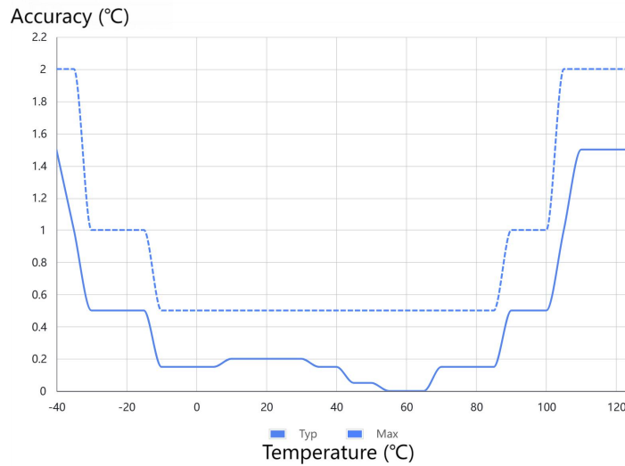
2. Accuracy corresponding to the temperature.
