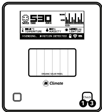
Assembled MClimate CO2 Display LoRaWAN®, top view
