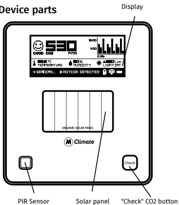
Assembled MClimate CO2 Display LoRaWAN®, top view
