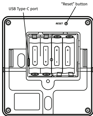
Disassembled MClimate CO2 Display LoRaWAN®, back view
