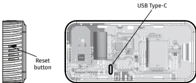
Assembled MClimate CO2 Display lite LoRaWAN®, side view
